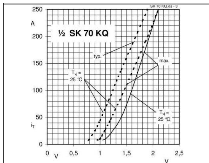
Fig. 3 On-state characteristics
